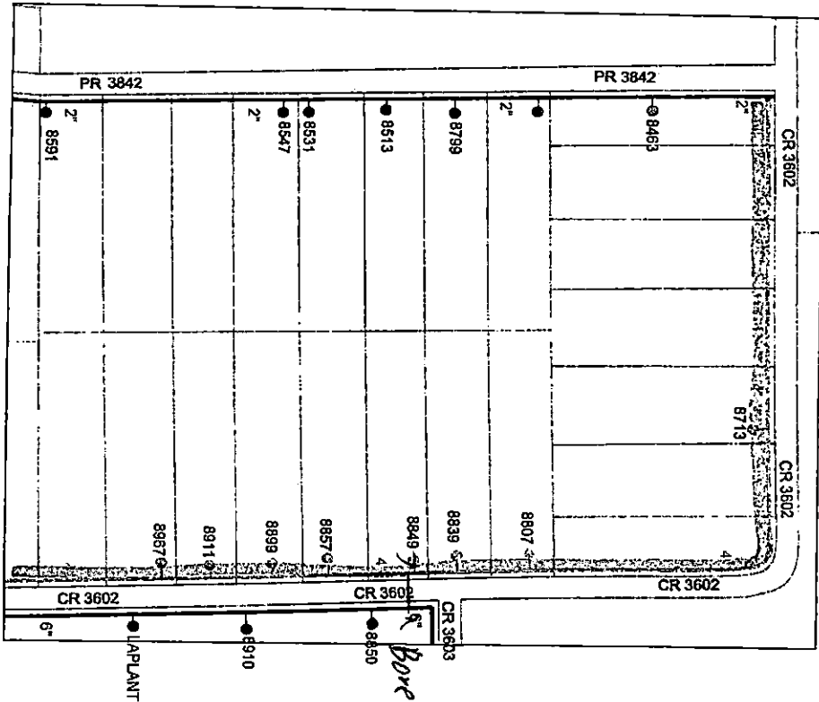
TRAIL DUST ESTATES EAST SCALE 1" = 250'
